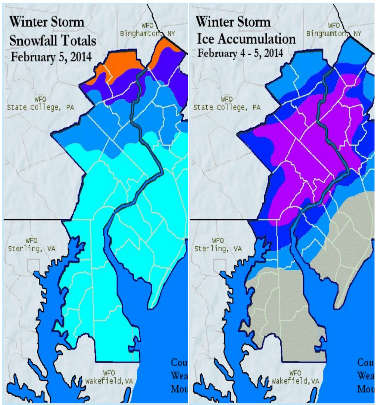
Storm Total Snow
