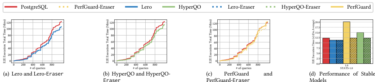
Figure 9: Performance of learned query optimizer on dynamic data.
