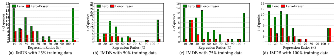
Figure 7: Performance of Lero-Eraser on queries with different training levels of regression.
