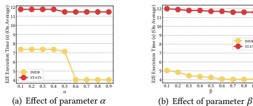
Figure 12: Effects of parameter \alpha and \beta .
