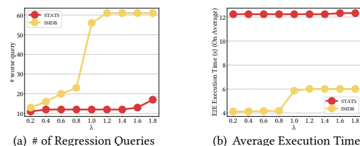
Figure 11: Effects of parameter \lambda .
