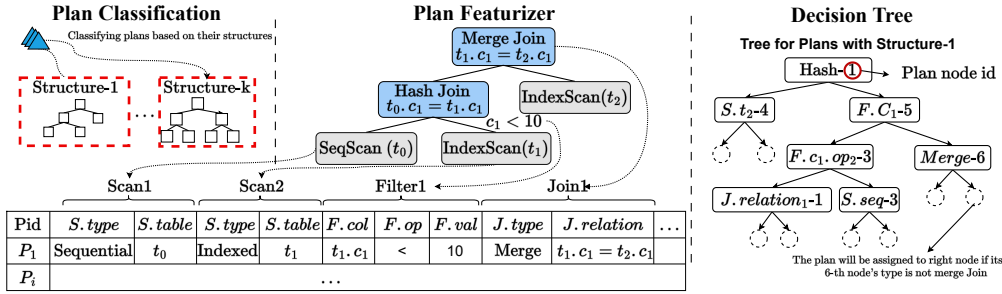
Figure 4: The example of the segment model. The left part is the plan classification process based on their structures. The middle part is the plan featurizer. The right part is a forest, where each tree represents the clustering model for a specific structure.
