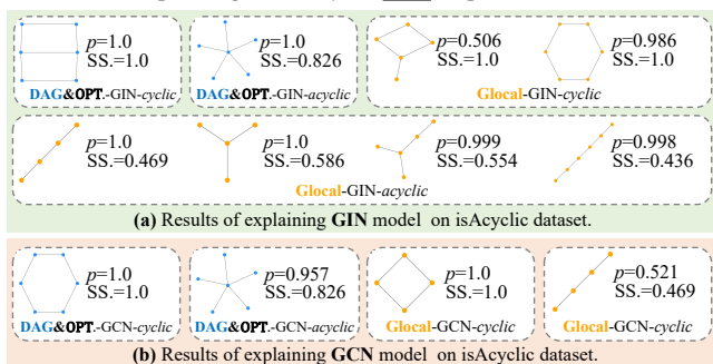
Figure 4: Results on the isAcyclic dataset. Visualization of the explanations with GNN score and Self-sup. (SS.) are reported. For both GNNs, OPT and DAG-Explainer give exactly the same outputs.
