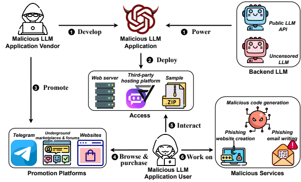
Figure 1: Malla workflow.
