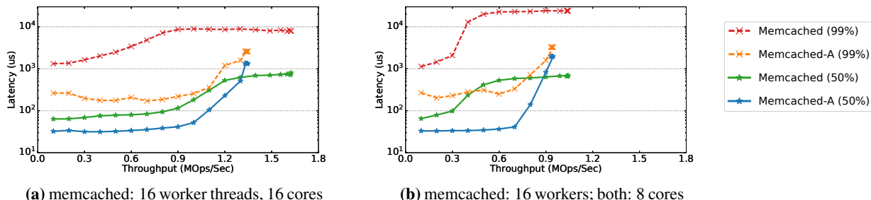
(a) memcached: 16 worker threads, 16 cores (b) memcached: 16 workers; both: 8 cores Figure 3: Median and 99th-percentile request latency as a function of achieved throughput for both memcached and memcached-A, under the Realistic benchmark. Each measurement ran for 30 seconds after a 5-second warmup. Y-axes use a log scale.
