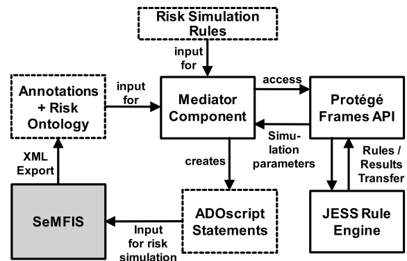
Fig. 6. Conceptual Architecture of Using SeMFIS together with Protégé and the JESS Rule Engine for Risk-based Simulations [14].
