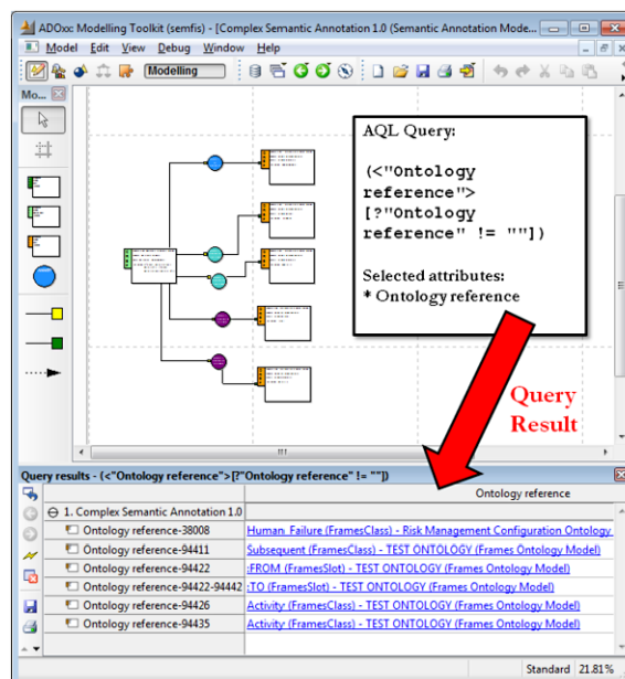
Fig. 3. Example for an AQL Query in SeMFIS retrieving Ontology Reference Elements in a Semantic Annotation Model Instance.
