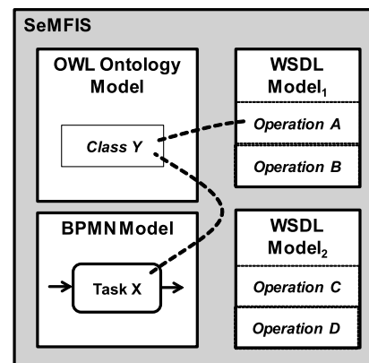
Fig. 7. Illustration of the Concepts Involved in Using SeMFIS for Semantic Discovery of Web Services.
