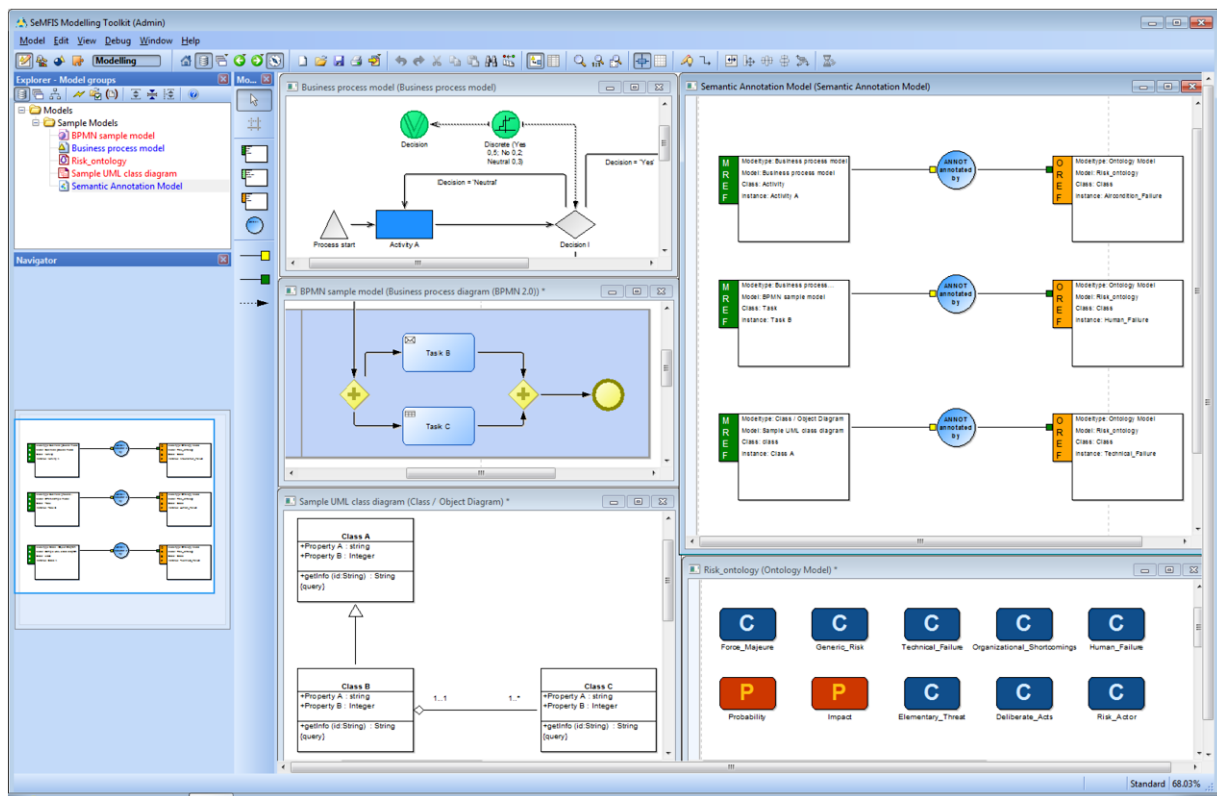
Fig. 2. Screenshot of SeMFIS showing Model Editors for a Business Process Models in ADONIS and BPMN notation, a UML Class Diagram, a Semantic Annotation Model, and an OWL Ontology Model.
