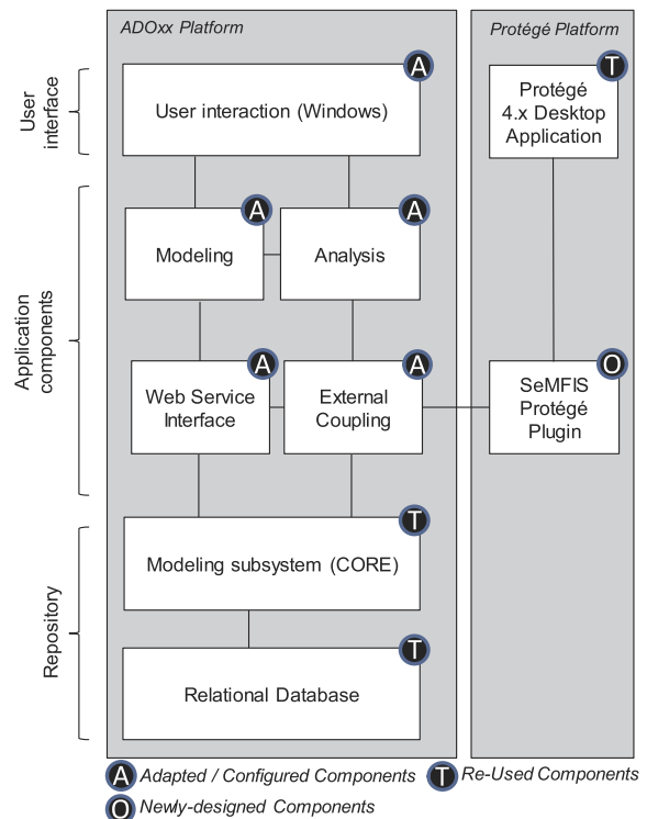
Fig. 5. SeMFIS Architecture based on ADOxx.
