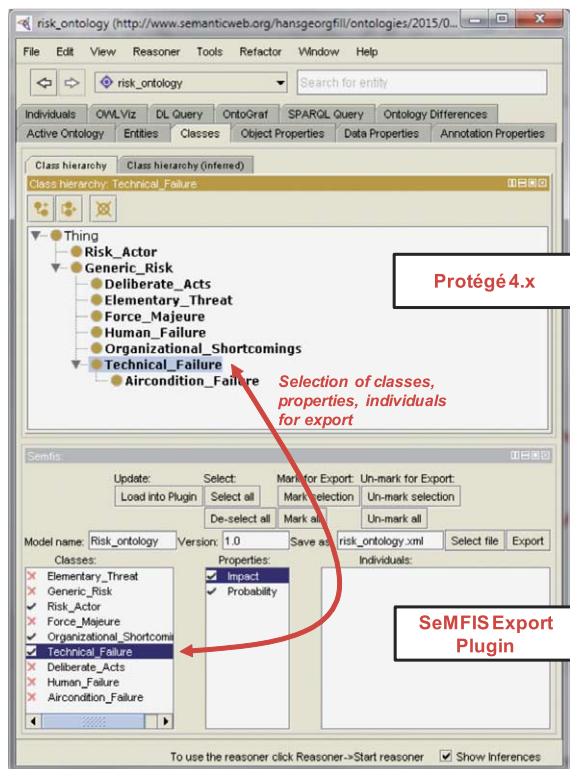
Fig. 4. Screenshot of the SeMFIS Protégé Plugin for Selecting Classes, Properties, and Individuals for Exporting them to SeMFIS.
