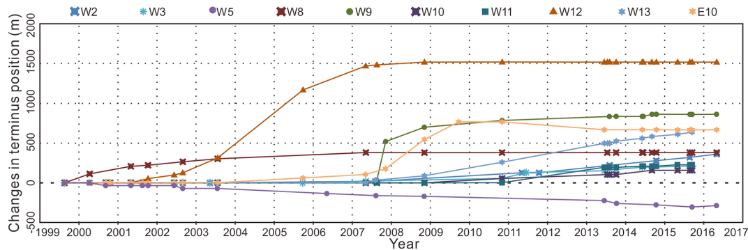
Figure 3. Changes in glacier terminus positions from 1999 to 2016 for 10 glaciers with detectable change.
