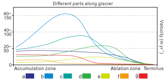
Figure 10. Conceptual characterization of the glacial motion pattern of surge-type glaciers in the Kingata Mountains. Profile a to Profile g indicate different stages during the active and quiescent phases of a surge-type glacier.
