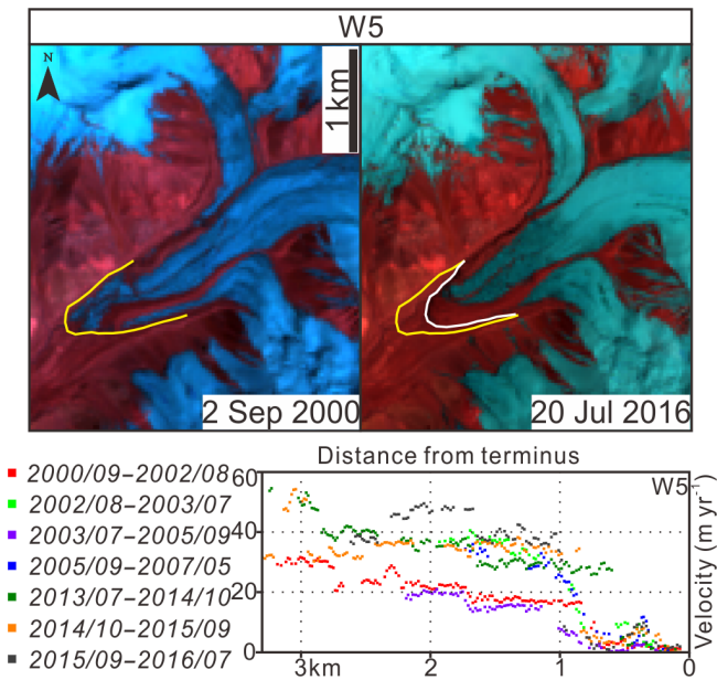
Figure 9. Comparison of W5 between 2000 and 2016 and its centre line annual-velocity profiles. The yellow line indicates its terminus position in 2000 and the white line indicates its terminus position in 2016.
