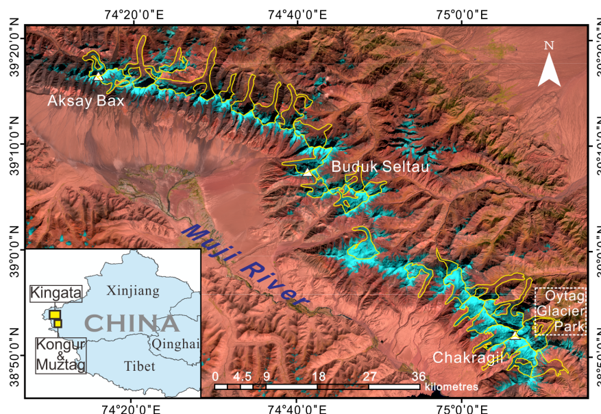
Figure 1. Landsat OLI image (bands 6, 5, and 4) of the Kingata Mountains acquired on 3 October 2014. Light blue areas represent bare ice, red-brown areas represent bare soil and rocks, and green areas represent grass or other vegetation. Glaciers with areas greater than 5 km 2 are highlighted by yellow lines.
