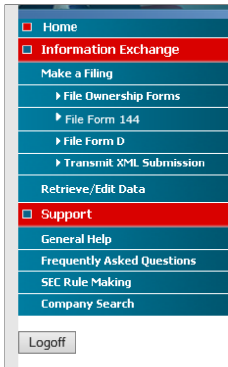
Figure 8-4: EDGAR Menu
