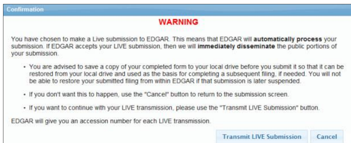
Figure 8-269: Confirmation Screen
