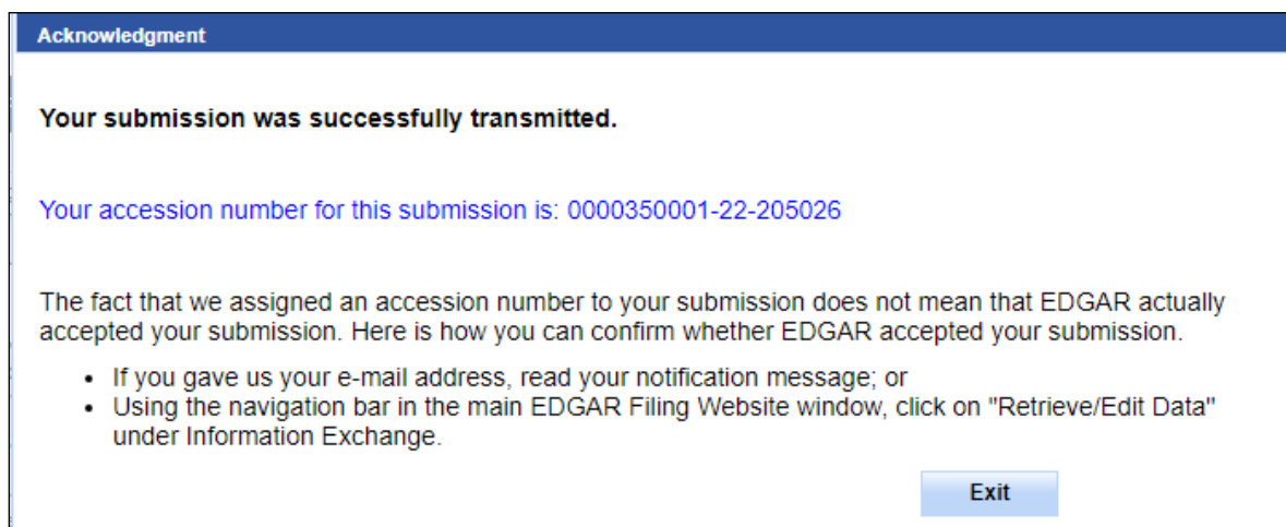
Figure 8-141: Acknowledgment Screen
