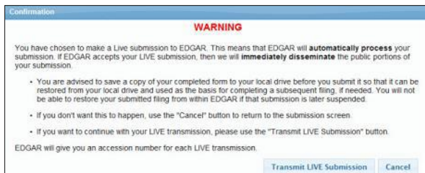
Figure 8-207: Confirmation/Warning screen
