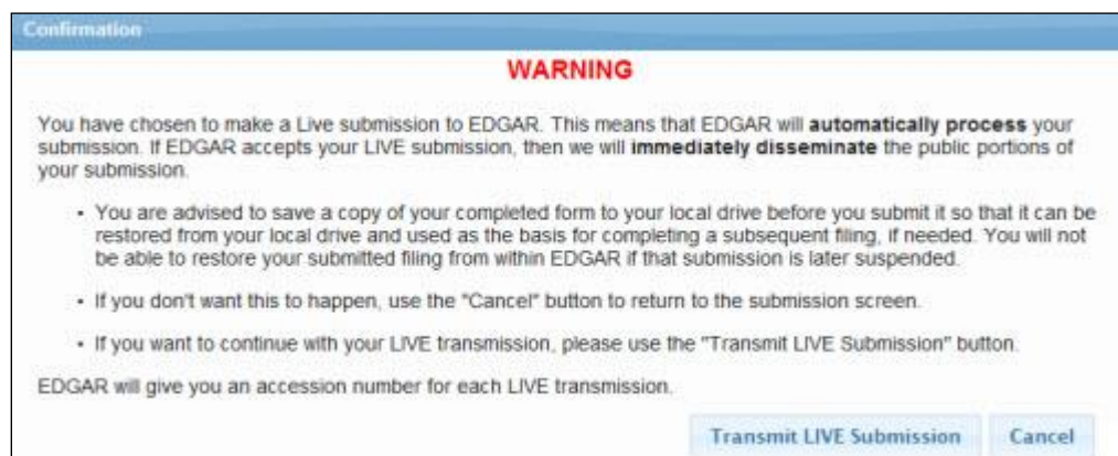
Figure 8-171: Confirmation Screen
