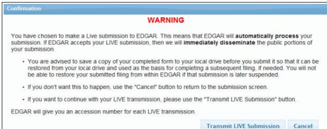
Figure 8-237: Confirmation/Warning Screen
