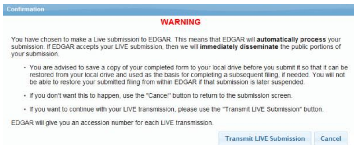
Figure 8-292: Confirmation Screen
