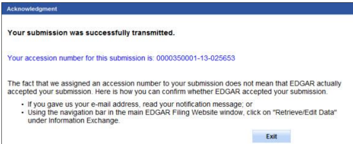
Figure 8-217: Acknowledgment Screen
