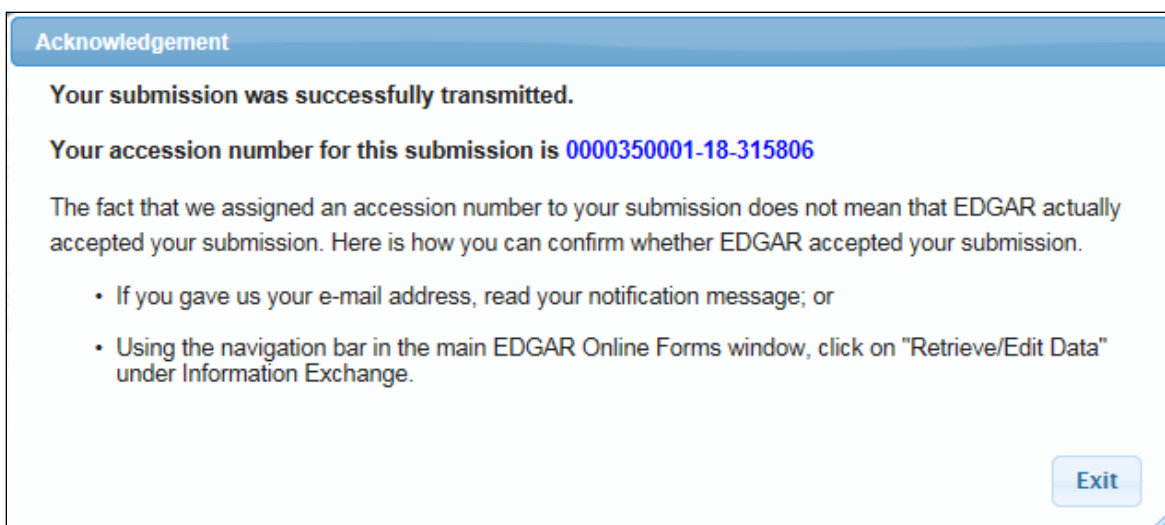
Figure 8-284: Acknowledgment Screen
