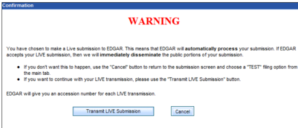
Figure 8-184: Confirmation Screen
