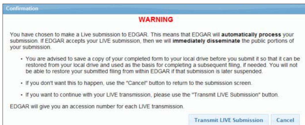
Figure 8-283: Confirmation Screen
