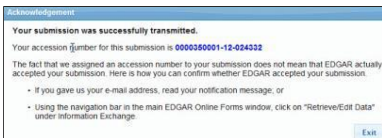
Figure 8-208: Acknowledgment screen
