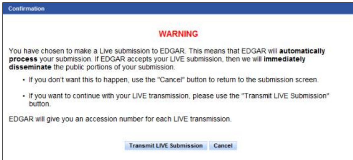
Figure 8-216: Confirmation Screen
