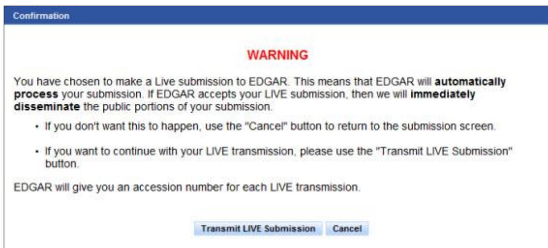
Figure 8-140: Confirmation Screen
