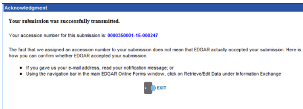
Figure 8-185: Acknowledgment Screen
