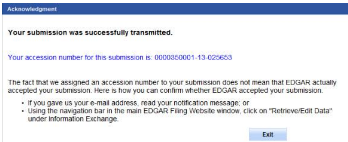
Figure 8-238: Acknowledgement Screen
