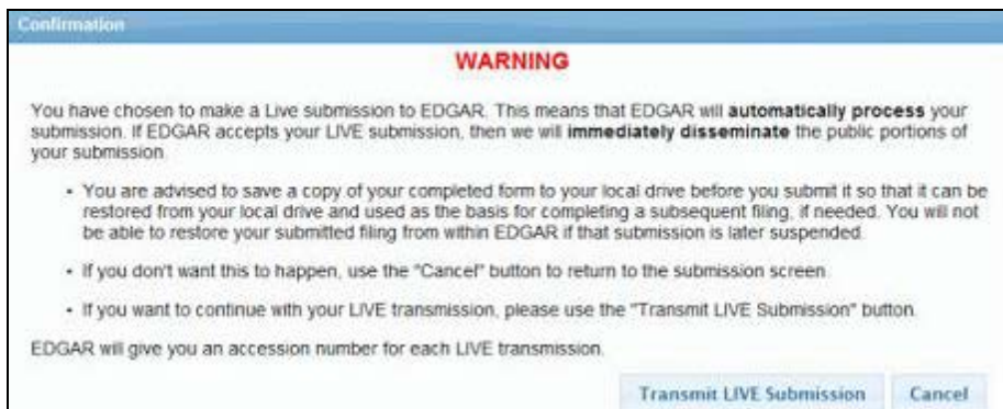
Figure 9-91: Confirmation/Warning screen
