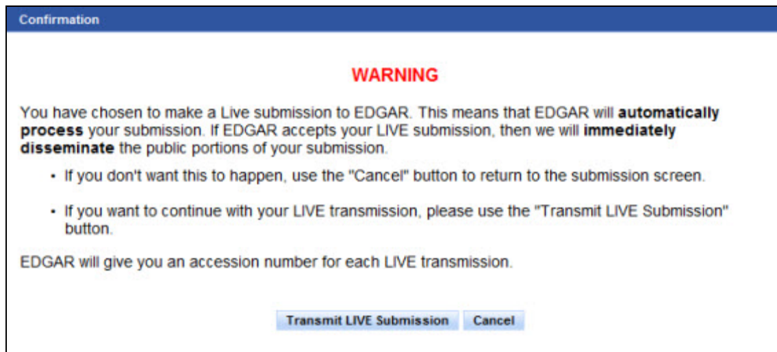
Figure 9-123: Confirmation Screen
