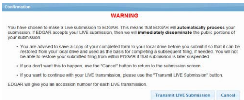
Figure 9-154: Confirmation Screen
