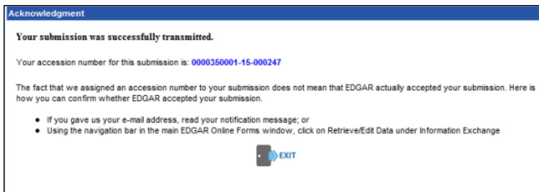
Figure 9-168: Acknowledgment Screen
