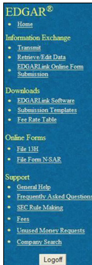
Figure 9-54: EDGAR Menu
