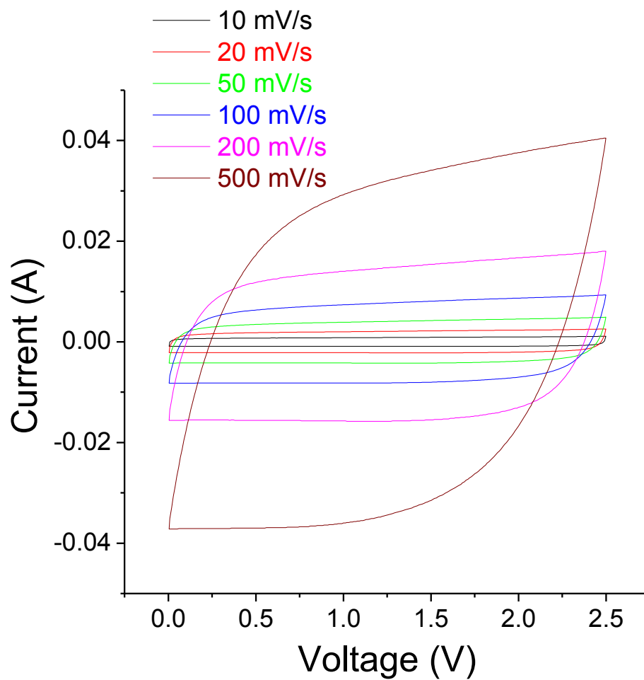
Fig. S2 Cyclic voltammograms of a symmetric supercapacitor based on N-OMC-800-3 at different scan rates (from 10 mV/s to 500 mV/s).
