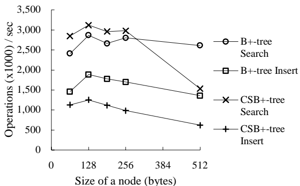
Figure 6. Performance of OLFIT with Varying Node Size
