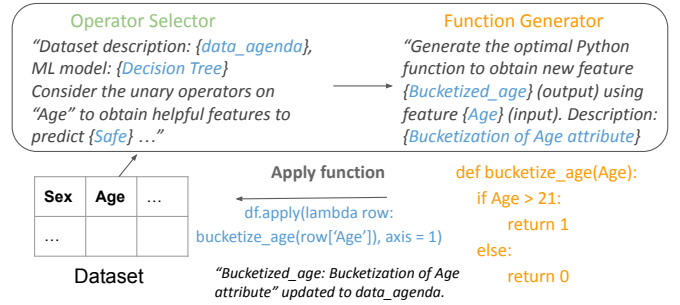
Figure 2: Illustrative example: constructing Bucketized Age .
