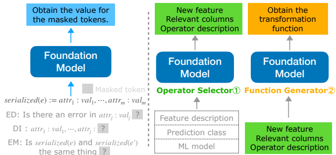
Figure 1: Comparison of row-level interactions to feature-level interactions.
