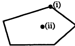
Figure 10. Possible relationships of R -point lying within R -cycle
