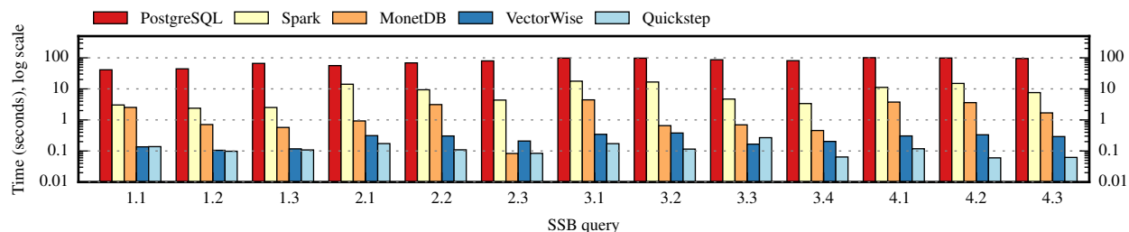
Figure 7: Comparison with denormalized SSB, scale factor 50.
