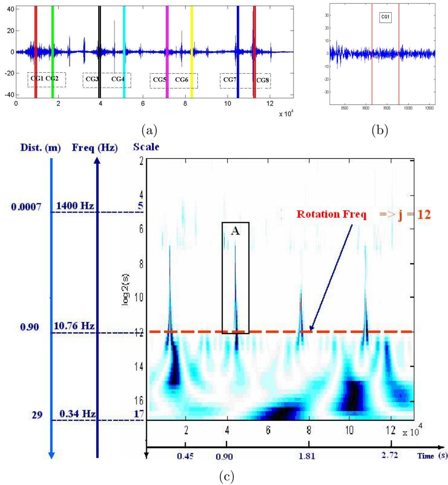
Fig. 2: (a) Whole temporal signal. (b) Zoom on the segment corresponding to pair of rollers CG1. (c) The time-scale representation (scalogram) of a signal.
