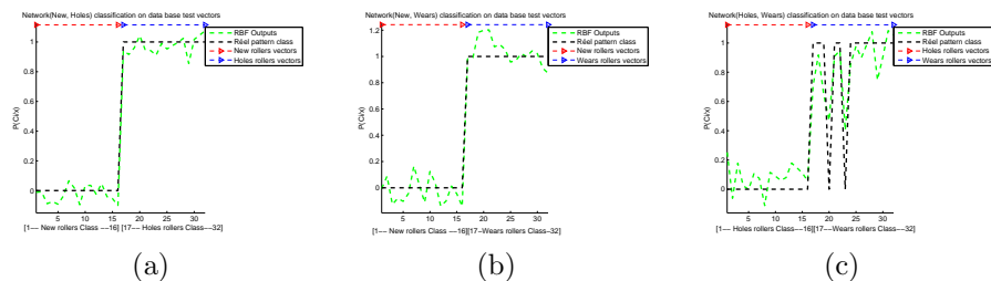
Fig. 3: RBF networks outputs : (a) new vs holes ; (b) new vs worn. (c) holes vs worn
