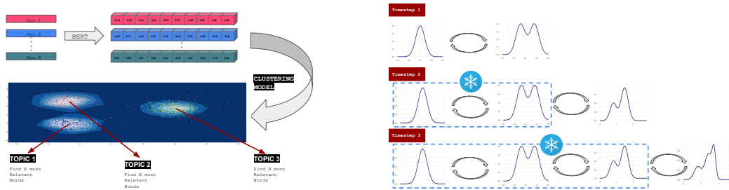
Figure 1: Panel (left) shows the working pipeline of a model like BERTopic, without considering the temporal aspect. Documents are transformed into embeddings, and clustering is performed. Each cluster represents a topic from which the N most representative words will be extracted.
