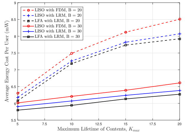
Fig. 4. Average energy cost vs. maximum lifetime of contents for cache capacities B = 20 and B = 30 when M_{max} = 8 , D_{max} = 15 , p_a = 0.25 .
