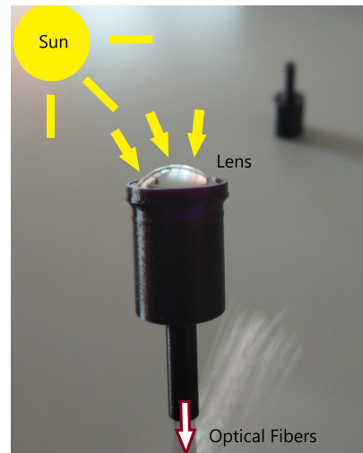
Figure 6: 3D printed light collector
