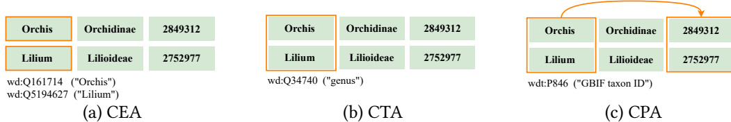
Figure 1: STA-tasks as defined by SemTab using a biodiversity example 5 .
