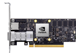
BlueField-2 DPU - 1x 200Gb/s HHHH form factor
