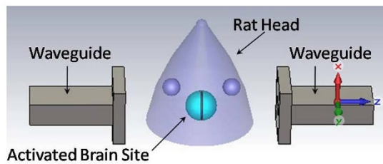
Figure 2 | Simulation setup, showing the 3D geometry of the simulated rat head, geometry and location of the simulated activated brain site, and waveguides assumed in the simulation, where the rat brain sizes were 16 mm from the left to the right, 12 mm from the front to the back, and 10 mm from the top to the bottom, the transmitting waveguide on the left was 10 mm away from the left side of the brain, the receiving waveguide on the right was 10 mm away from the right side of the brain, and each of the waveguides was a rectangular hollow metallic waveguide of 7.11 mm × 3.56 mm.
