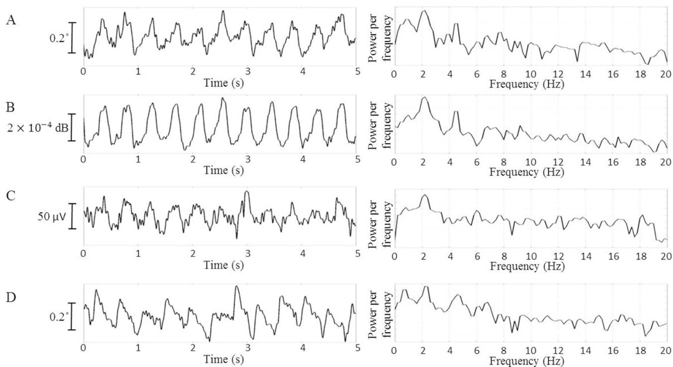
Figure 5 | Experimental results, where (A) shows the variation of the phase change of the EM wave propagating through the rat brain as well as the spectral density distribution. (B) The variation of amplitude change of the EM wave propagating through the rat brain and the spectral density distribution. (C) The EEG signal measured on the rat and the spectral density distribution. (D) After the EEG electrodes were removed from the rat, the variation of the phase change of the EM wave propagating through the rat brain and the spectral density distribution.
