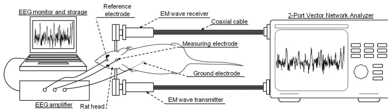
Figure 4 | Experimental setup, where a rat, anaesthetised with ether, was placed with the head centred in between the transmitting waveguide and receiving waveguide of an Agilent N5230A PNA-L 2 Port Vector Network Analyzer that was transmitting, receiving and analysing the variation of the EM wave propagating through the rat brain via an EEG electrode attached on the lambda, a reference electrode attached to the eye socket, and a ground electrode attached on the body. The electrodes were connected to an ANT EEG amplifier for acquiring EEG simultaneously with the EM wave measurement. This figure was drawn by TCW.
