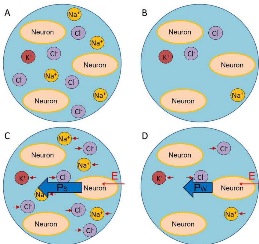
Figure 1 | The neuronal activation at a brain functional site gives rise to immense transmembrane ion flows, varying the ion concentration of the extracellular fluid at the functional site, and therefore, varying the permittivity of the fluid. (A) When the neurons are in synchronised depolarisation, their membranes pump sodium ions out and largely increase the ion concentration in the surrounding extracellular fluid. (B) When the neurons are in synchronised repolarisation, many sodium ions rush into the neuronal cell bodies and largely reduce the ion concentration of the extracellular fluid. (C) Under an applied electric field, E (shown with a small red arrow indicating the field direction), a strong polarisation density, P_S , is formed in the extracellular fluid at the functional site when the neurons are in synchronised depolarisation and result in a high ion concentration of the extracellular fluid. (D) Also, under the applied electric field, E (shown with a small red arrow indicating the field direction), a weak polarisation density, P_w , is formed in the extracellular fluid at the neuronal activation site when the neurons are in synchronised repolarisation and result in a low ion concentration of the extracellular fluid.
