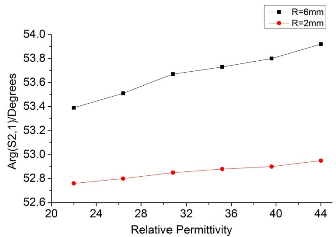
Figure 3 | Simulation result showing the variation in the phase change \arg(S_{2,1}) of the 30 GHz EM wave propagating through an activated brain site vs the variation of the relative permittivity of the dielectric at the brain site. The approximately spherical, activated brain site with a radius R = 6 mm exhibited the variation of EM wave phase change, which increased from 53.39° to 53.92° when the relative permittivity of dielectric at the activated brain increased from 22 to 44. The approximately spherical, activated brain site with a radius R = 2 mm exhibited the variation of EM wave phase change, which increased from 52.76° to 52.95° when the relative permittivity of dielectric at the activated brain increased from 22 to 44.
