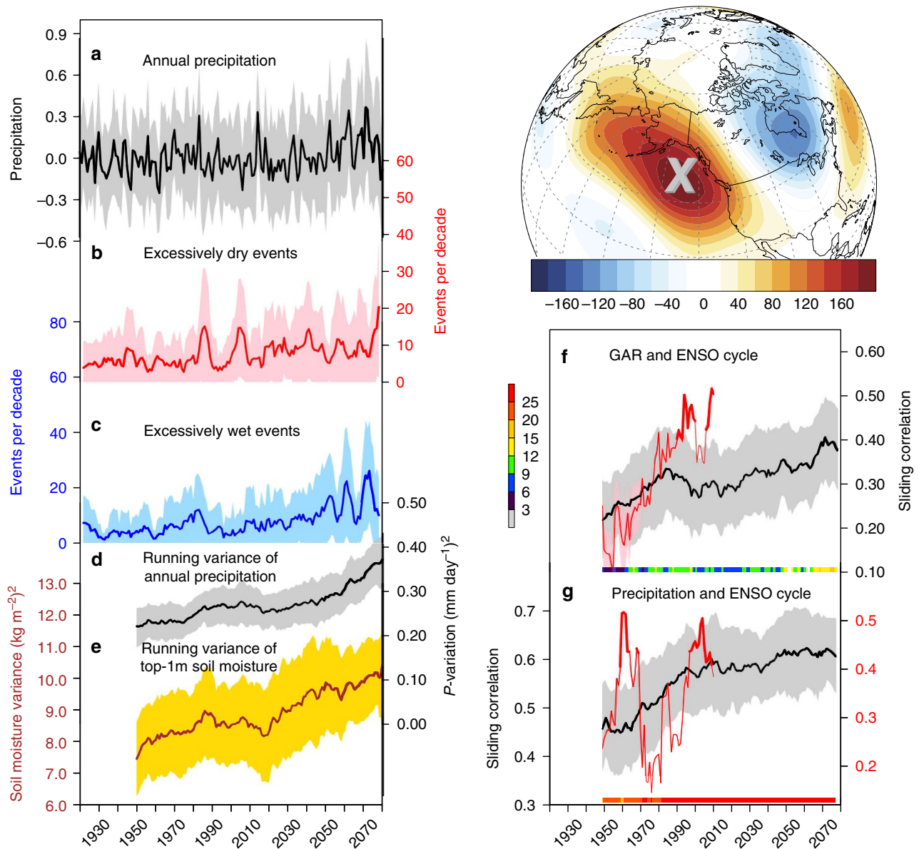
Figure 1 | Changing water cycle extremes in California simulated by CESM1. (a) Annual mean precipitation, (b) excessively dry events per year with 5-year running average (see text and Methods section), (c) excessively wet events per year with 5-year running average, (d) 30-year running variances of annual precipitation and (e) 30-year running variances of annual soil moisture in the top 1 m of soil layers averaged over California. Solid lines indicate a 30-member ensemble mean of CESM1, while shaded areas indicate model spread; roughly 50% of the ensemble members are within the shaded areas (see Methods section). The inset map atop (f) shows the November 2013–January 2014 geopotential height anomaly at 200 hPa depicting the GAR and the center location for the GAR index (cross). Right panels: the multivariate correlations between the Niño-3.4, Niño-3.4( Y + 1 ) and (f) Gulf of Alaska Ridge (GAR) index and (g) annual precipitation averaged for water year in California, defined as October to September in the following year, within a running 30-year window during the NDJ season. The red line in f is the multivariate correlation ( r ; see Methods section for formula) derived from the reanalysis data and that in g is from observed SST and precipitation (see Methods section). Note that the y axis scale is different in g for model (black; left) and for observation (red; right). Statistical significance of the multivariate correlations is given as a colour bar in g,f showing the number of the ensemble members that are significant with 90% confidence based on the F-test. Similarly, thicker red lines represent the years with 90% significance.
