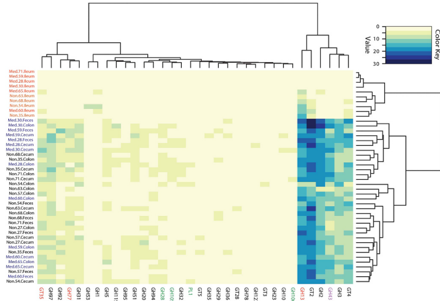
Figure 2 CAZy family abundances per sample. Heatmap depicts the relative abundances of several CAZy families (x-axis) by sample (y-axis). Sample names are coded by treatment status (Med, medicated; Non, non-medicated), pig number and sampling site. Relative abundance was calculated as the fraction of reads with statistically significant sequence similarity to sequences in a particular CAZy gene family, multiplied by a scaling factor (11 000). CAZy families are colored for functions highlighted in the results: starch breakdown (red), and the digestion of PCW components such as pectin (green) and hemicellulose (purple).
