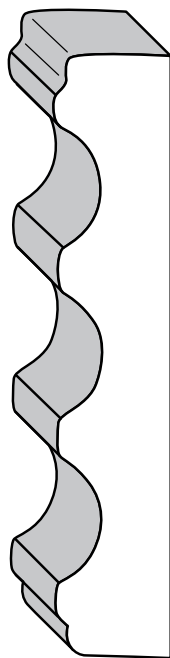
305 Fluted Casing 1 1/16" x 3 1/2" Clear Pine (P305) Oak (O305)
