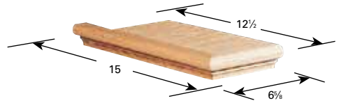
8071 Right-Hand and Left-Hand False Tread Cap
