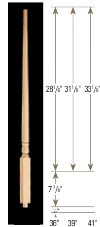
5015 1 1/4" Baluster PR501536 PR501539 PR501541
