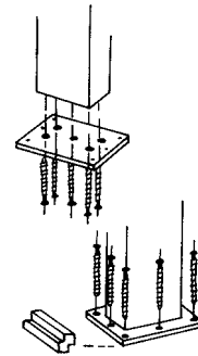
3006 Newel Plate Kit w/ Trim
