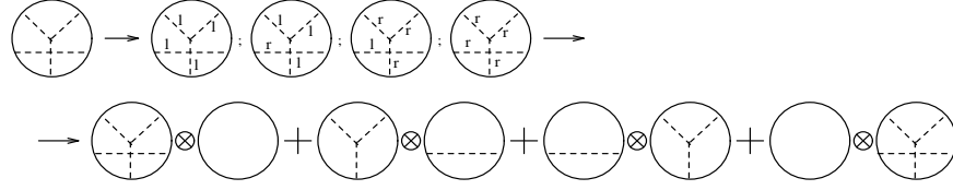
Figure 12. Computing \Delta(\text{trivalent vertex}) .
