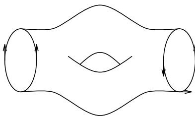
Figure 5. A marked surface with two boundary components
