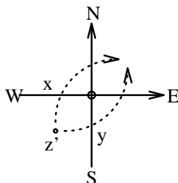
Figure 7. The graph SW and the two ways of getting from it to NE . Notice that z' is perpendicular to the plane and therefore appears as a single dot.
