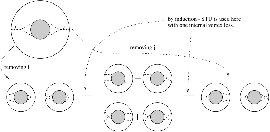
Figure 8. The consistency proof
