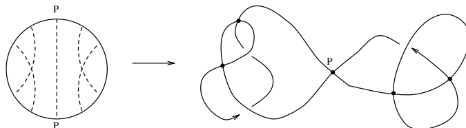
Figure 6. The knot corresponding to a diagram having an isolated chord. The ends of the isolated chord are mapped to the point P .
