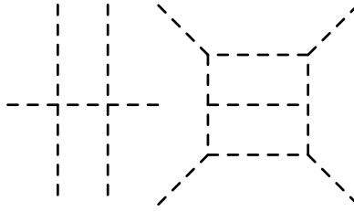
Figure 4. A Chinese Character (CC) of degree 8. As in the case of CCDs, all trivalent vertices are oriented counterclockwise and all apparent vertices of valency higher than 3 are not vertices at all. This CC has four connected components.
