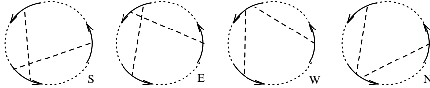
Figure 1. The diagrams S , E , W , and N . (The dotted arcs represent parts of the diagrams that are not shown in the figure. These parts are assumed to be the same in all four diagrams)
