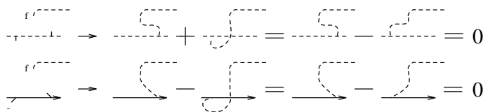
Figure 10. Grouping by arcs
