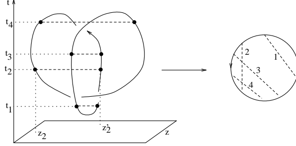
Figure 13. m = 4 : a knot K with a pairing P and the corresponding chord diagram D_P . Notice that D_P = 0 in \mathcal{A}_{\mathbb{C}}^r due to the isolated chord marked by 1.
