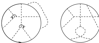
Figure 2. A Chinese Character Diagram (CCD) together with the conventional way of drawing it, as outlined in the text.
