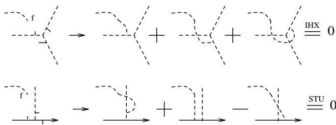
Figure 11. Grouping by vertices
