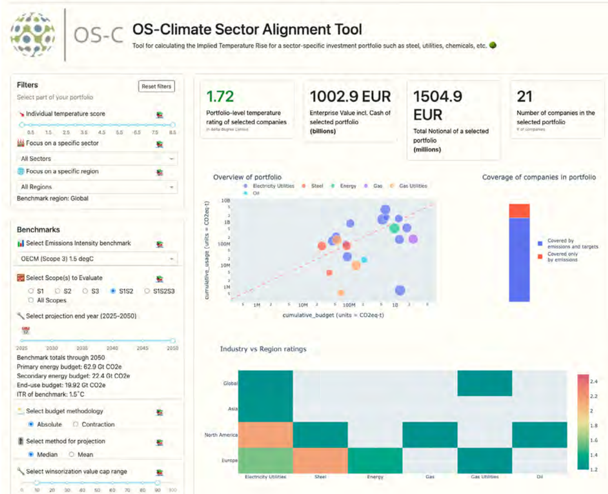
A sample portfolio of companies in different regions and sectors. Companies at or below the dashed red line (or rendered in green in the heatmap) have an alignment with 1.5°C 2050 targets.
