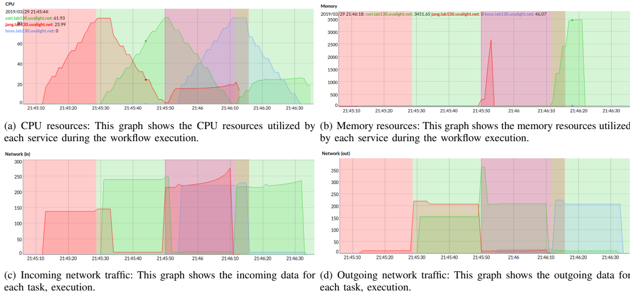
Fig. 6. Combined results after parsing the workflow, querying the provenance file and querying the relevant resource usage. All sub-figures highlight each service execution with a separate color which corresponds to the colors shown in Figure 5(b)
