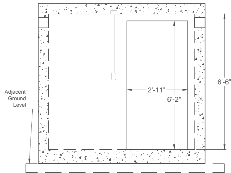
FRONT ELEVATION
