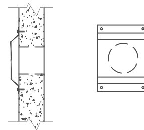
VENT DETAIL
