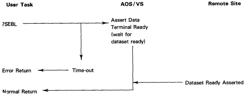
Figure 14-8. ?SEBL System Call, Point-to-Point
