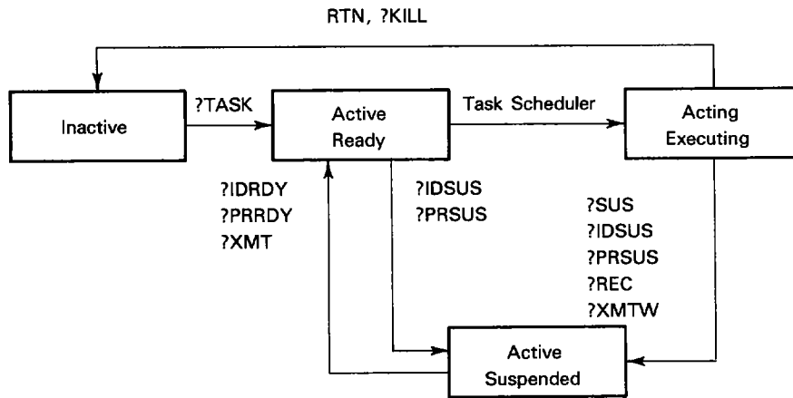
Figure 7-1. Task States
