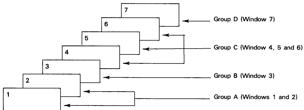
Figure 6-5. Grouping Windows
