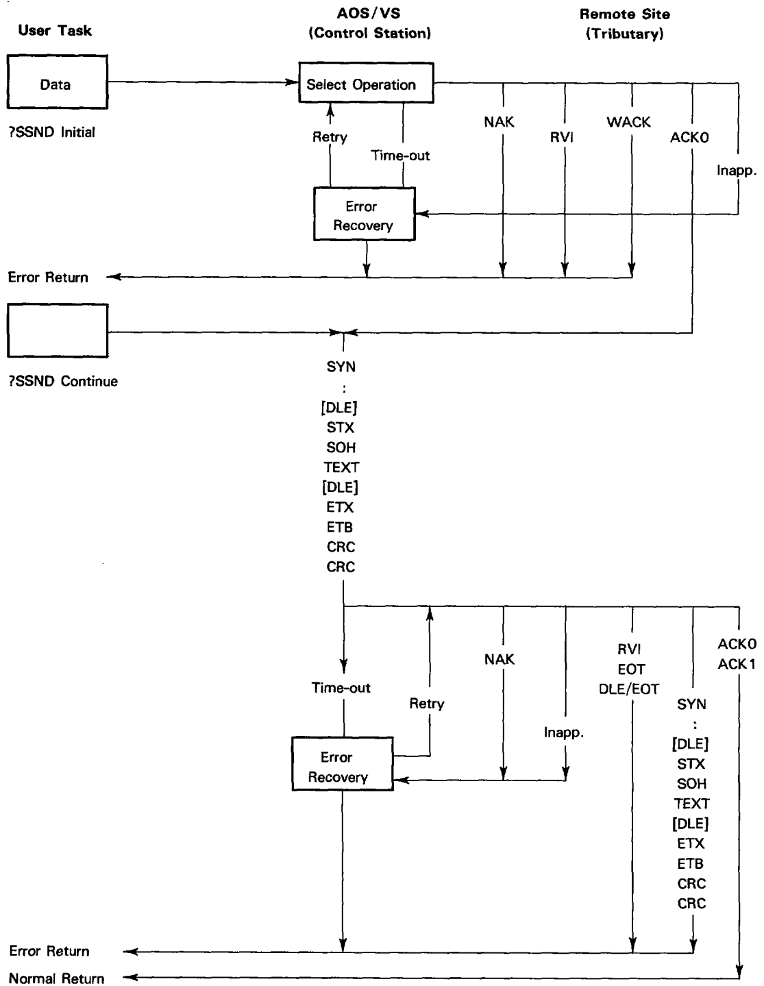
Figure 14-5. ?SSND System Call, Multipoint Control Station
