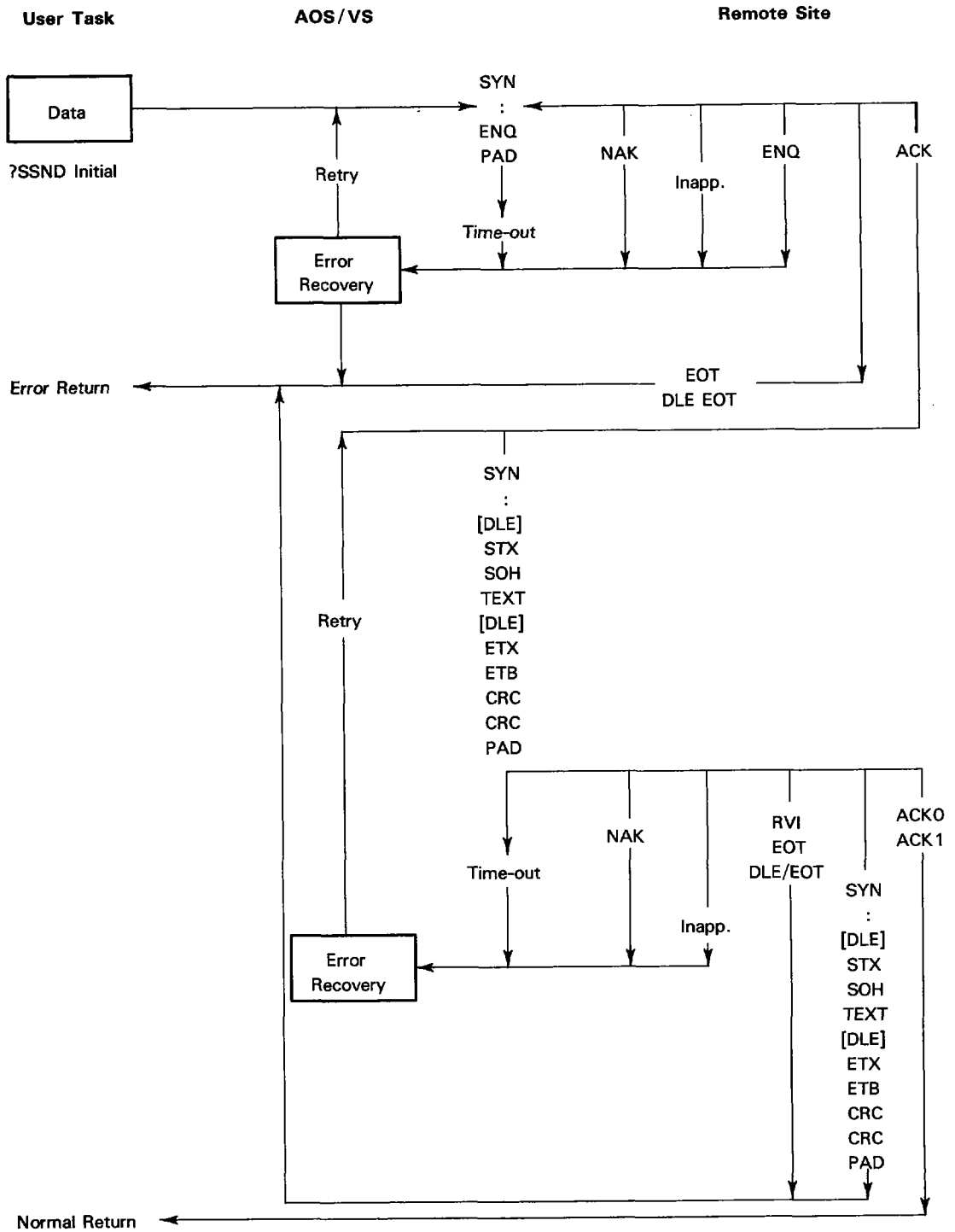
Figure 14-2. ?SSND System Call, Initial, Point-to-Point
