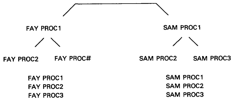
Figure 3-3. Process Names
