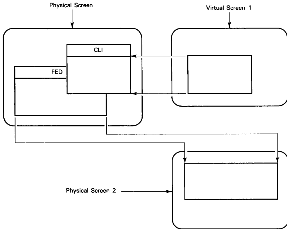
Figure 6-3. Overlapping Windows
