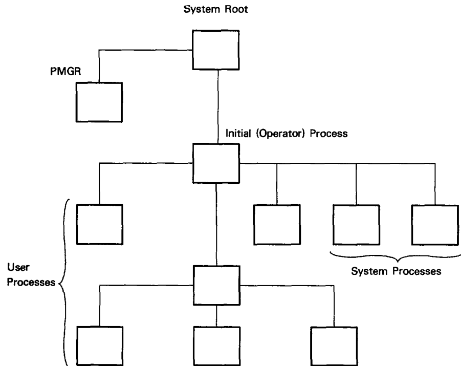
Figure 3-2. Process Hierarchy
