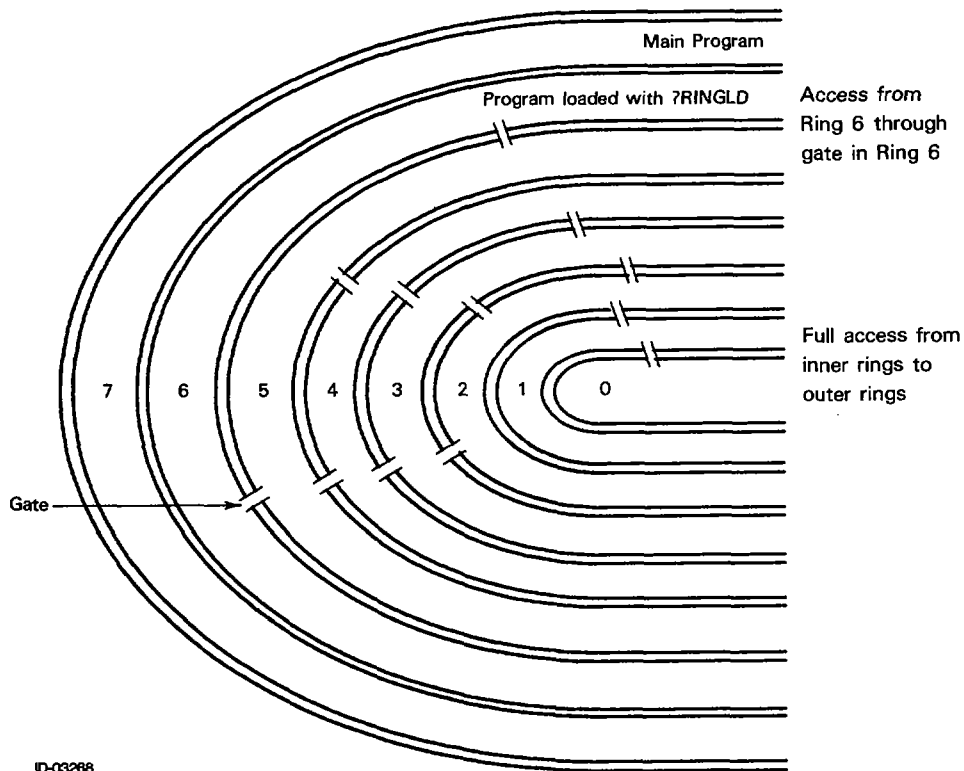
Figure 3-5. Ring Structure
