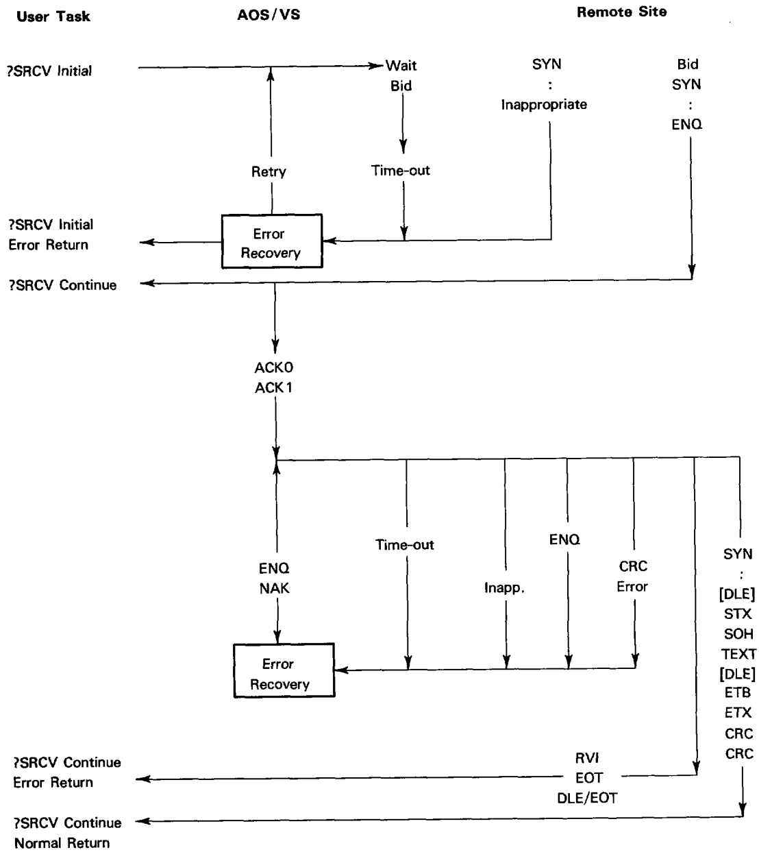
Figure 14-4. ?SRCV System Call, Initial and Continue, Point-to-Point
