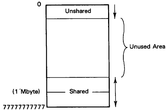
Figure 2-3. Memory Context
