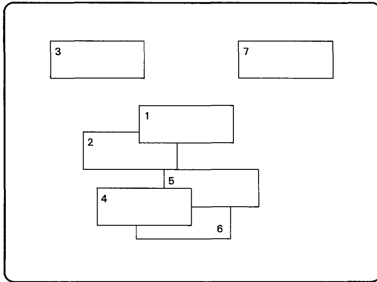
Figure 6-4. Window Priorities
