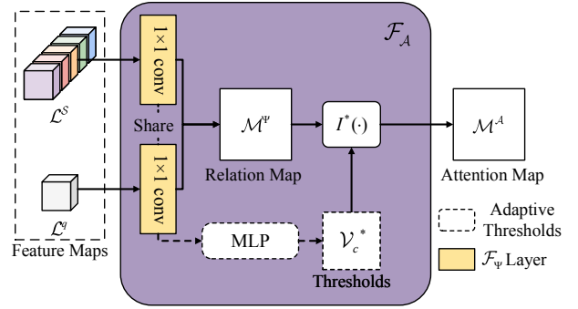
Figure 2: The framework of adaptive episodic attention module \mathcal{F}_A . Through this module, we obtain episodic attention by \mathcal{L}^Q and \mathcal{L}^S . The components with dashed lines generate adaptive thresholds \mathcal{V}_c^* , which is a fixed manual defined hyperparameter in TL-Net.
