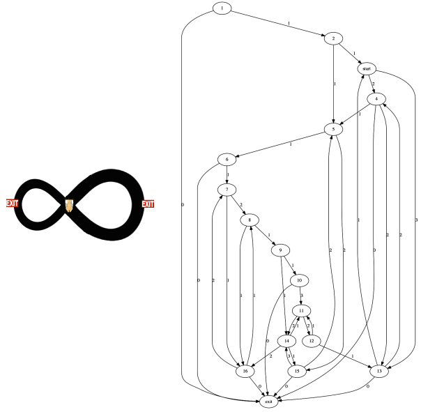
Figure 1: The Double Loop environment (left) and the Pacman Labyrinth (right)
