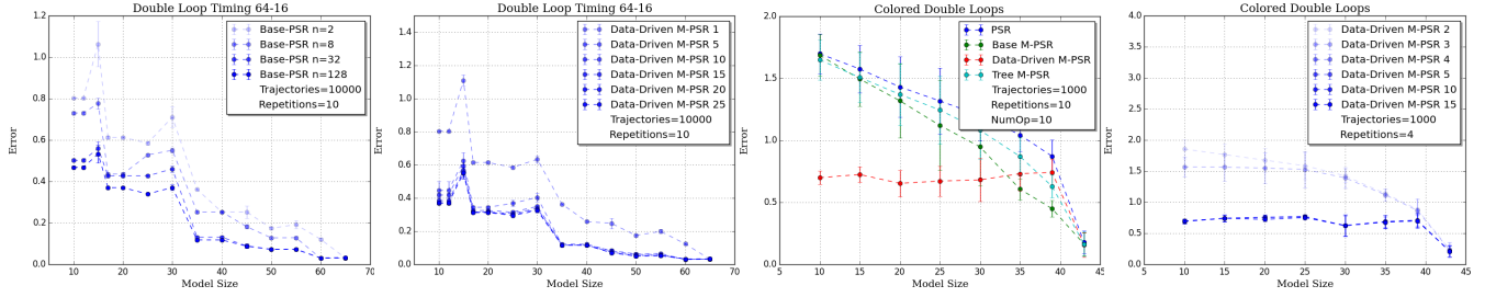
Figure 4: (1) Effect of exponent in Base M-PSR (Double Loop 64-16) (2) Effect of the number of operators (Double Loop 64-16) (3) Effect of model size (Colored Double Loop 27-17) (4) Effect of the number of operators (Colored Double Loop 27-17)
