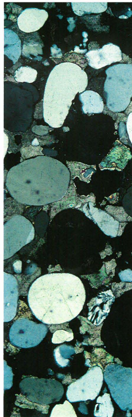
Well-rounded quartz grains are cemented with calcite crystals in this sandstone cored from a depth of 652 feet in western Sioux County. Cross-polarized light, magnified 29x.
