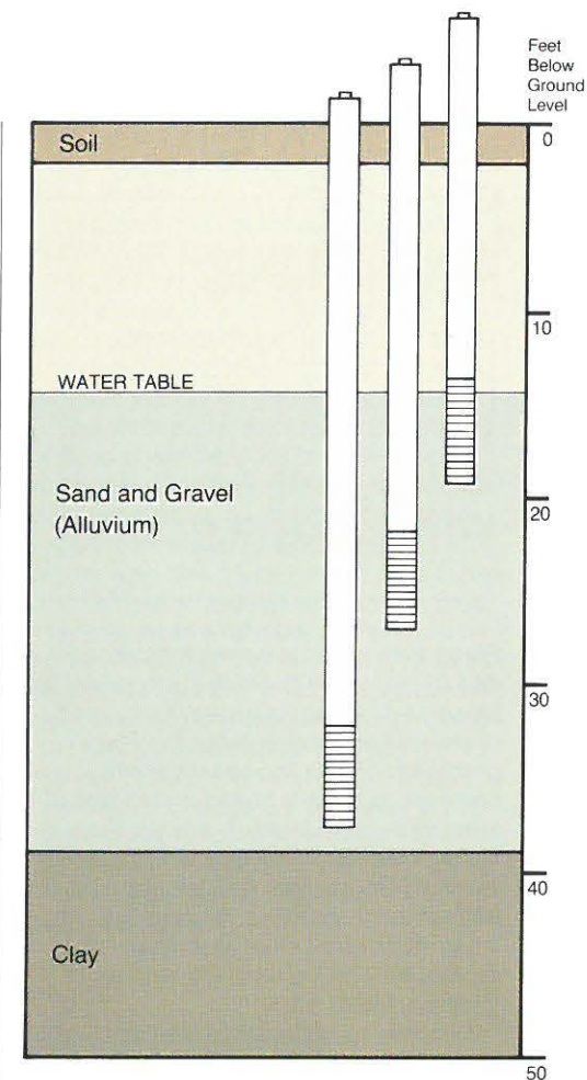
Nested wells placed to different depths within an aquifer enable vertical sampling of a site's water quality characteristics.
