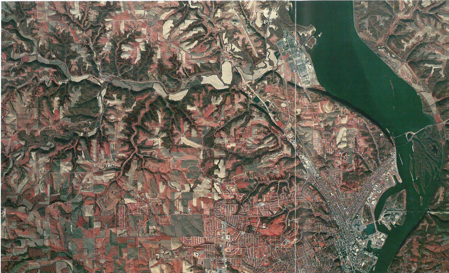
This color-infrared photo shows the city of Dubuque, Lock and Dam 11, and the Little Maquoketa entering the Upper Mississippi River at Peru Bottoms, a Savanna Terrace remnant. The Little Maquoketa formerly flowed southeasterly through Dubuque. Its abandoned channel, known as Couler Valley, may be traced in the photo.
