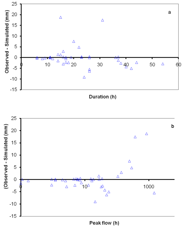
Fig. 6. Model error (observed minus simulated runoff) versus duration ( a ) and observed peak flow (log-scale) ( b ) for the 38 events in Wadi Koutine.
