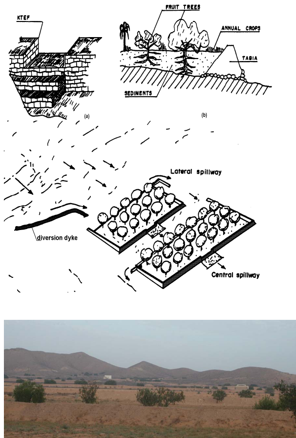
Fig. 2. Upper: scheme of the Jessr components (a spillway, b side view) (adapted from El Amami, 1984). Lower: scheme of a tabia with natural impluvium (adapted from Alaya et al., 1993). In the photo: tabias are seen in the front (piedmont area) and jessour are found in the talwegs of the mountains in the back.
