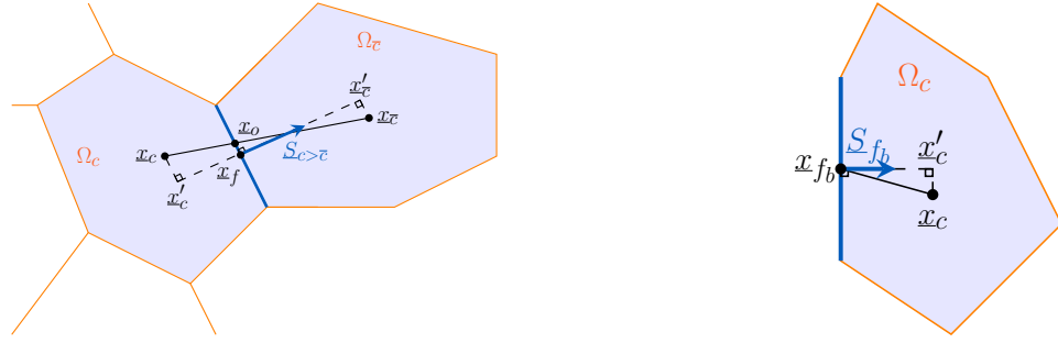
Figure IV.A.1: Definition of the geometric entities for internal (left) and a boundary faces (right).
