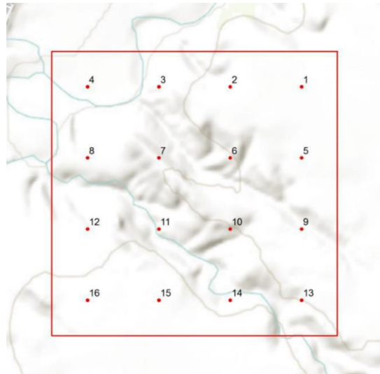
Figure 1. Diagram of a grid (red outline) and points (red dots). Grids may also be referred to as “transects” or “surveys”. Individual points should always be referred to as “points” (not “surveys”).
