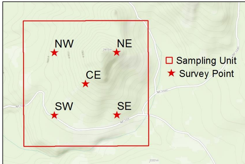
Figure 2. 1-km 2 sampling unit containing five survey points, used to survey for Mexican Spotted Owl site occupancy in 2017 in the US Forest Southwestern Region.
