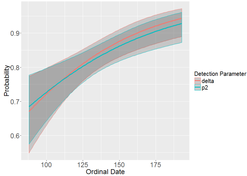
Figure 5. The relationship between date and p^2 and \delta as estimated by the most parsimonious model of site occupancy by Mexican Spotted Owls in the US Forest Southwestern Region, 2014-2017. The shaded regions represent 95% confidence intervals around the estimate. The ordinal date of April 1 is 100. Delta ( \delta ) is the probability that a pair of owls is detected in a site during a survey and p^2 is the probability that occupancy is detected for a site during a survey, given that the site contains a pair of owls. The effect of date on p^1 was not included in the most parsimonious model and is not presented here.
