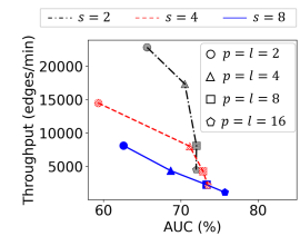
Figure 7: AUC w.r.t throughput.
