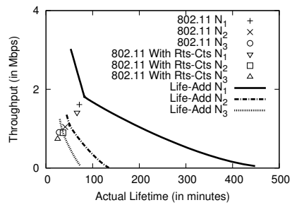
Fig. 4: Simulation results for single AP networks with heterogeneous devices.
