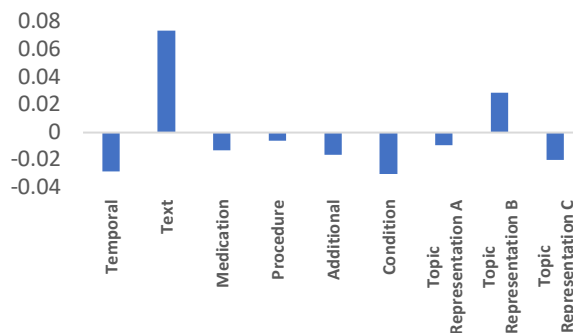
Figure 5. B-Pref prediction changes on simulated data for selected characteristics. Values represent change in predicted B-Pref using a simulated dataset with all permutations of the four word-based query parameters and the six binary taxonomy flags. All other values are held constant while varying the characteristic listed.
