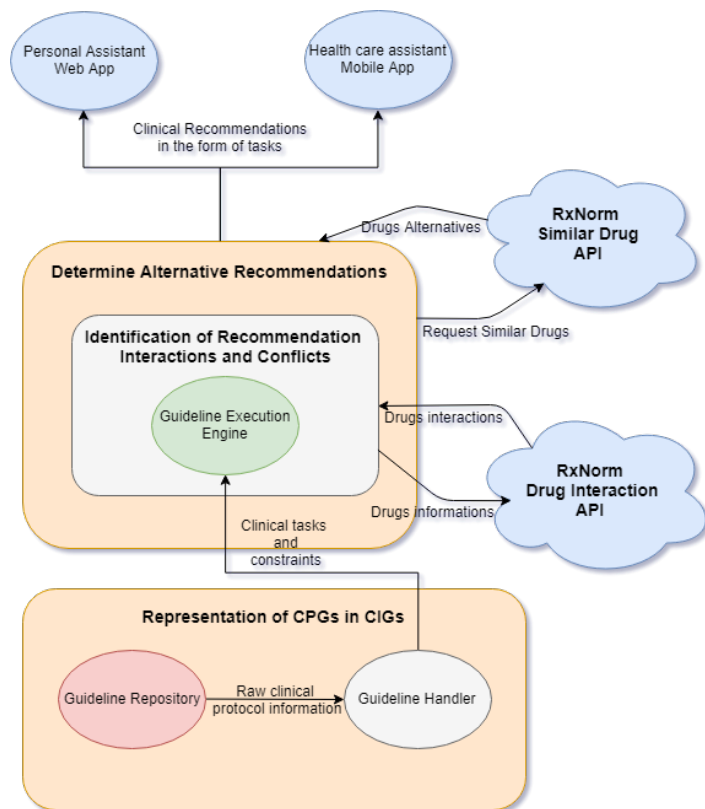
Figure 1: Architecture of CompGuide system
