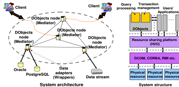
Figure 2: DObjects System Architecture
