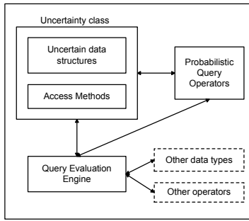
Figure 1: The architecture of U-DBMS
