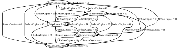
Figure 6: Visualization of aggregate control-flow for Hadoop's execution. Each vertex represents a TaskTracker. Edges are labeled with the number of ReduceCopies from the source to the destination vertex.
