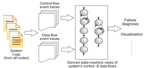
Figure 1: SALSA's approach.
