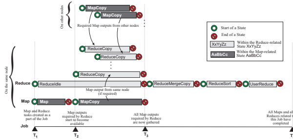
Figure 7: Visualizing Hadoop's control- and data-flow.
