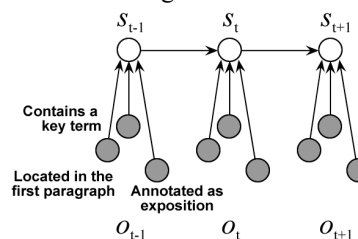
Figure 2 Graphical model for CMMs.
