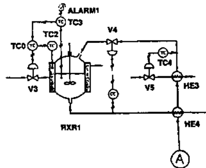
Figure 4: Chemical reactor subsystem (Stephanopoulos 84)
