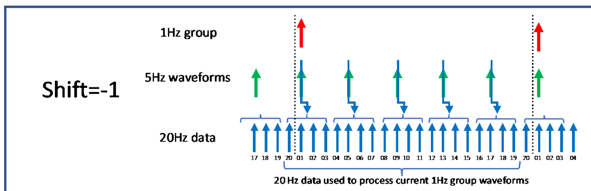
Figure 6. 20 Hz tracking data shift for combination with 5 Hz C Band waveforms.
