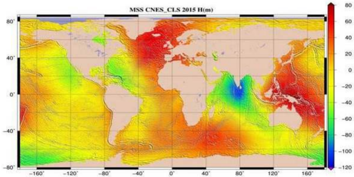
Figure 26. Mean Sea Surface MSS_CNES-CLS15 (m).
