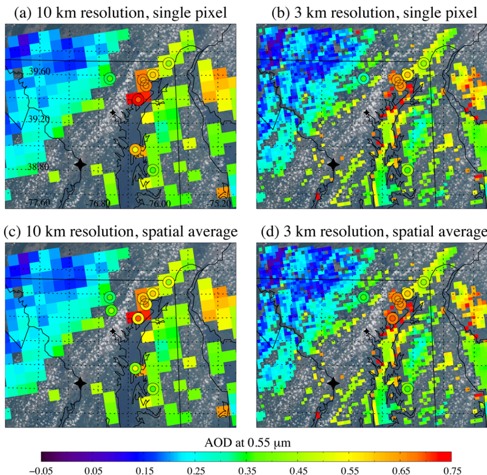
Fig. 1. AOD at 0.55 \mu\text{m} observed by MODIS-Aqua on 21 July 2011 at 18:30 UTC is plotted at the 10 km resolution (a and c) and 3 km resolution (b and d). MODIS/SP collocations are plotted in the circles. In (a–d), the inner circle is the SP temporally averaged AOD, which is an average of \geq 2 SP measurements within 30 min of MODIS overpass. In (a) and (b), the outside circle is the AOD of the MODIS pixel containing the SP site. In (c) and (d), the outer circle is the spatial average of a MODIS AOD in a 5 \times 5 pixel box around the SP station. Only land pixels with a QA = 3 are used in the collocation. Washington D.C. is shown with the large black star and Baltimore, MD is shown with the small black star. The true color image, created from the MODIS red, green and blue bands, is shown in the background.
