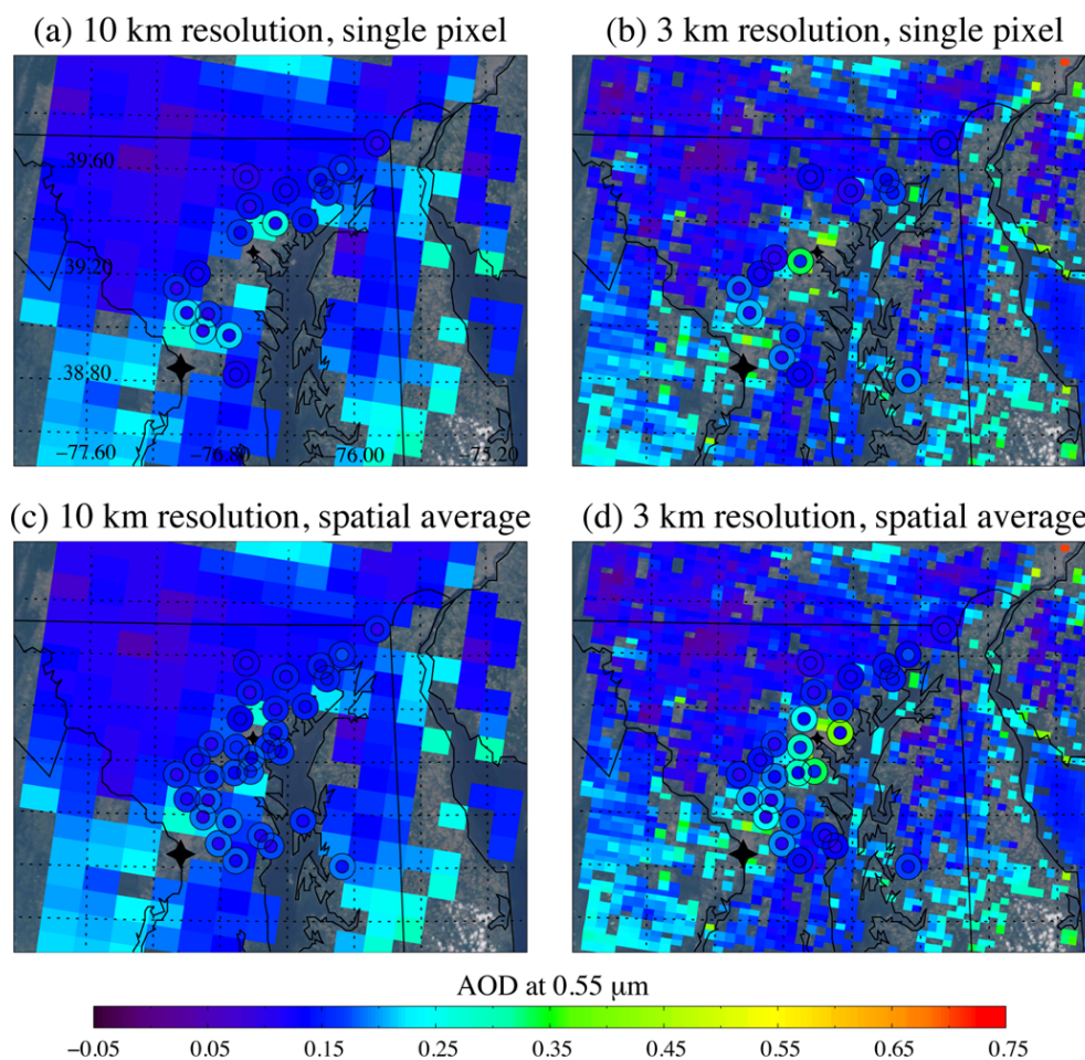
Fig. 2. AOD at 0.55 \mu\text{m} observed by MODIS-Terra on 1 July 2011 at 15:35 UTC is plotted at the 10 km resolution (a and c) and 3 km resolution (b and d). MODIS/SP collocations are plotted in the circles. In (a–d), the inner circle is the SP temporally averaged AOD, which is average of \geq 2 SP measurements within 30 min of MODIS overpass. In (a) and (b), the outside circle is the AOD of the MODIS pixel containing the SP site. In (c) and (d), the outer circle is the spatial average of a MODIS AOD in a 5 \times 5 pixel box around the SP station. Only land pixels with a QA = 3 are used in the collocation. Washington D.C. is shown with the large black star and Baltimore, MD is shown with the small black star. The true color image, created from the MODIS red, green and blue bands, is shown in the background.
